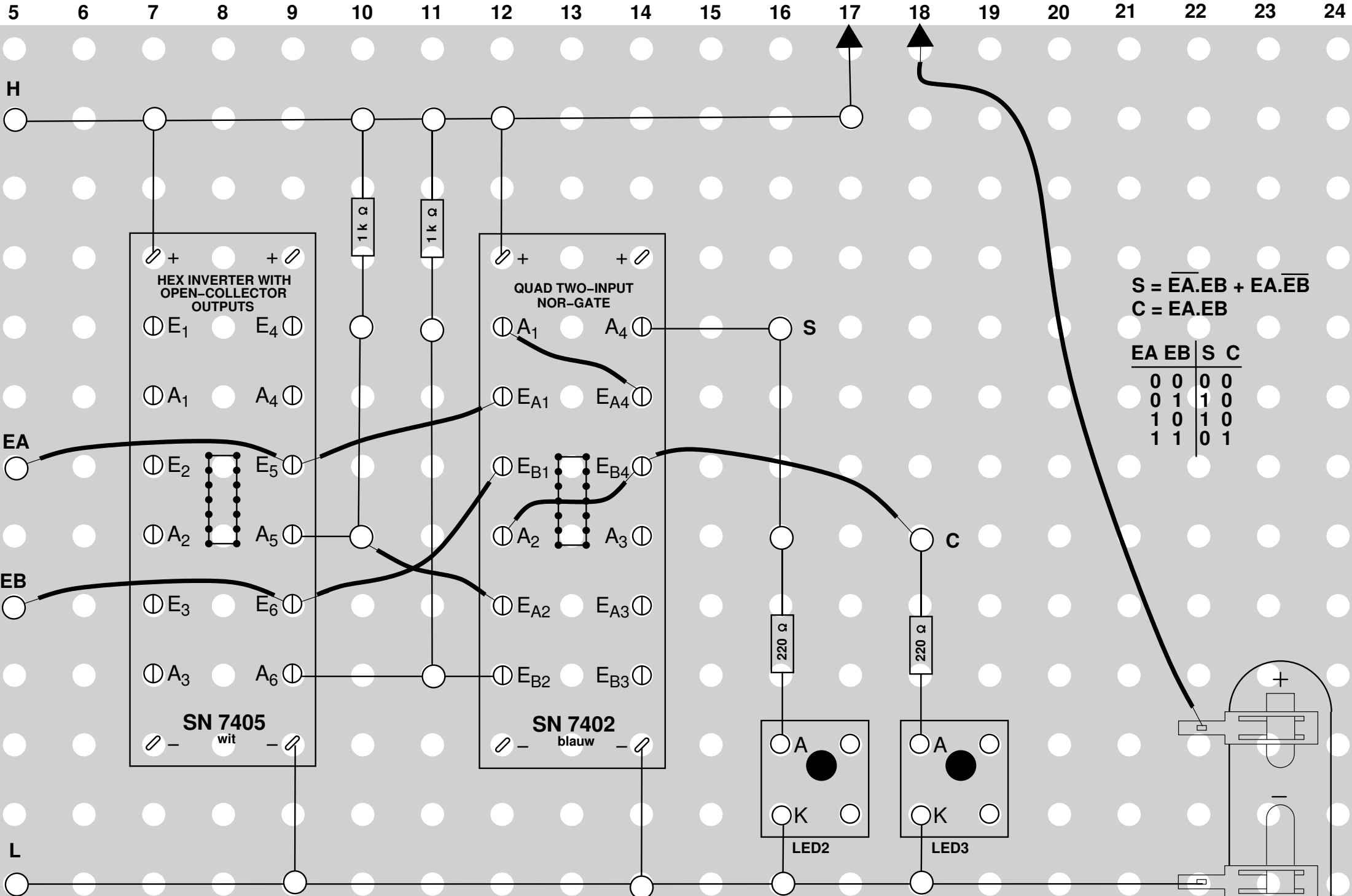
4.10.20. 1-bit half-adder
